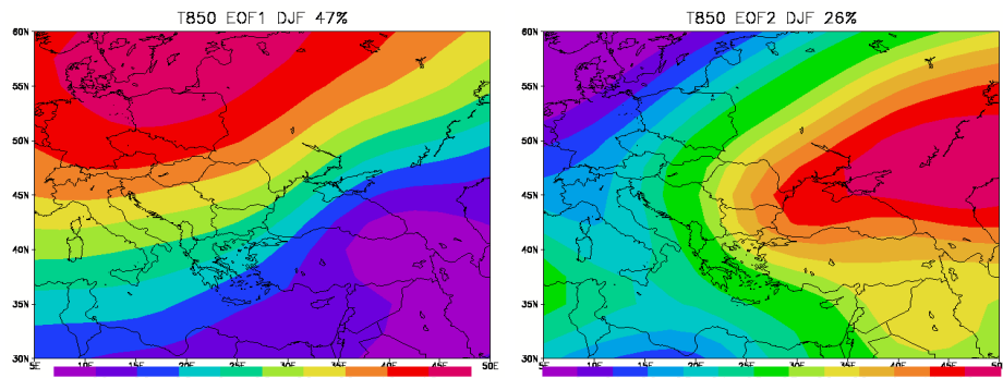
Fig. 10 - The pattern of the first (EOF1) and second (EOF2) T850 EOF configurations for the winter season
