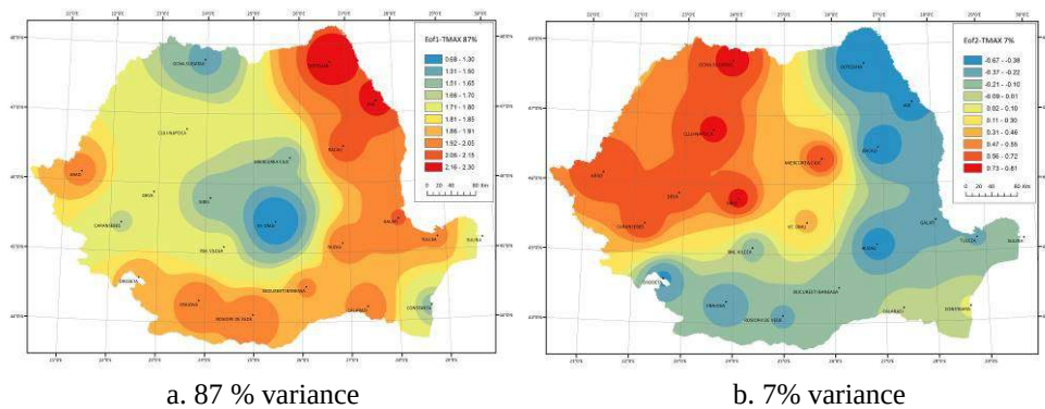
a. 87 % variance b. 7% variance Fig. 4 - The first two EOF patterns of the mean maximum air temperature values during the winter season, in Romania
